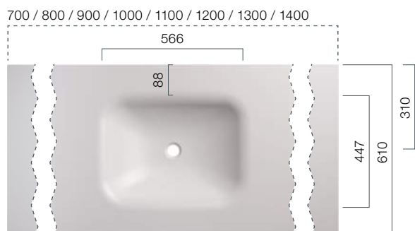
Position Basin: Central; Depth: 120 mm
