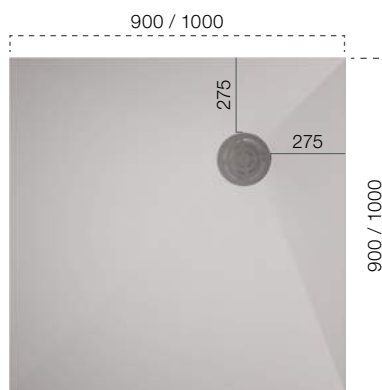
XERO Square – Drain central
